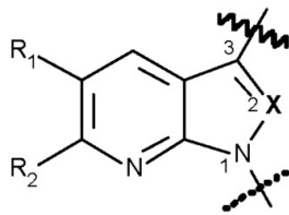
5-Aza-Derivate
