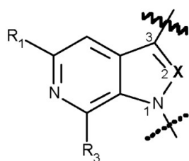
6-Aza-Derivate
